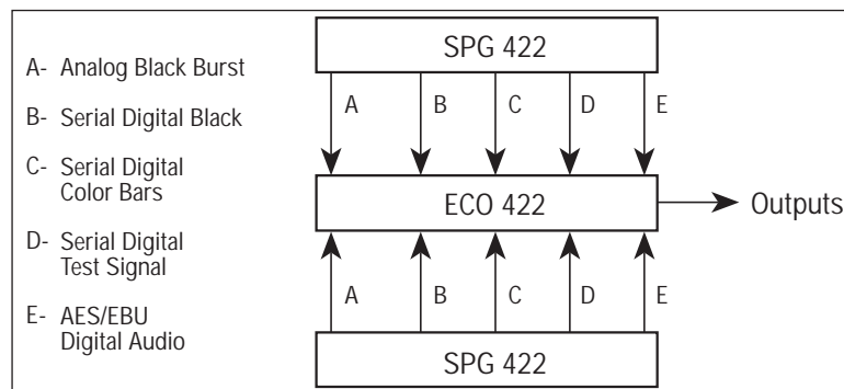
Component digital master sync system. The ECO 422 provides eleven user configurable signal channels, each consisting of primary and backup inputs and an output.
